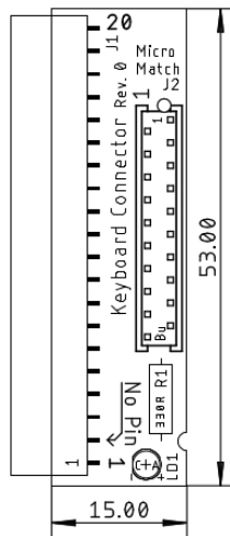
Figure 2: Dimensions of the PCB
